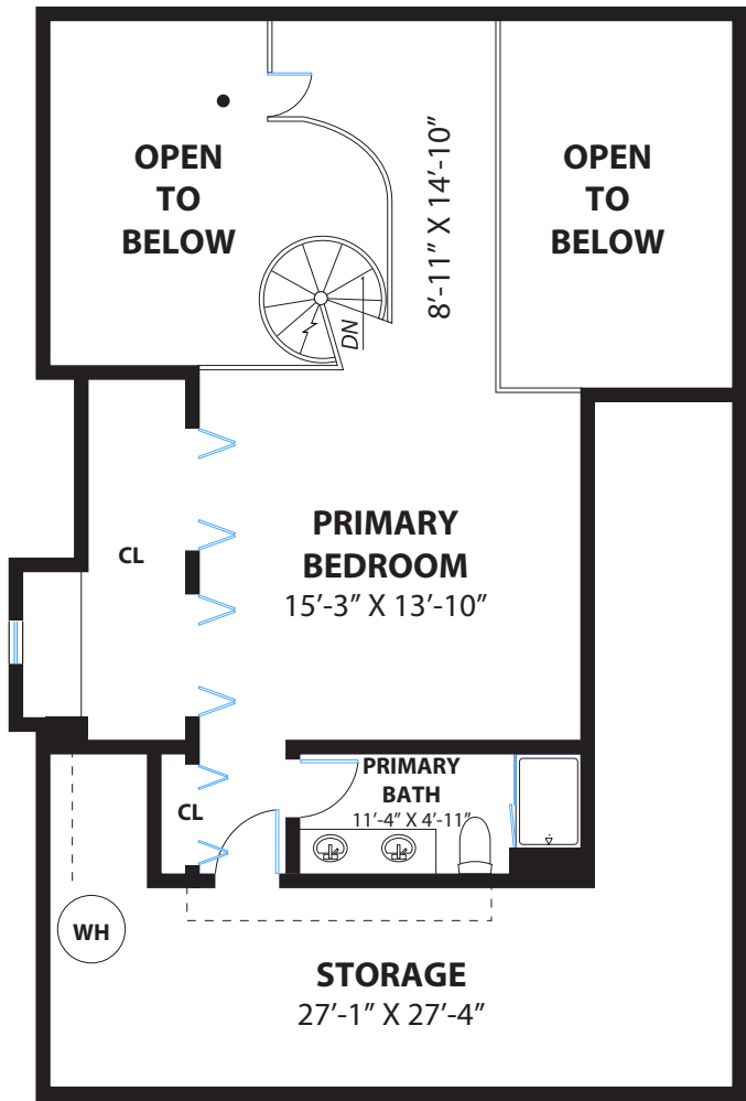
UPPER LEVEL
